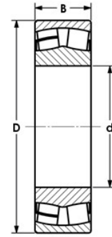
Straight Bore
