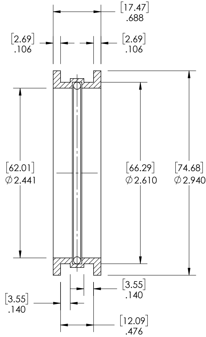
SECTION VIEW A-A
