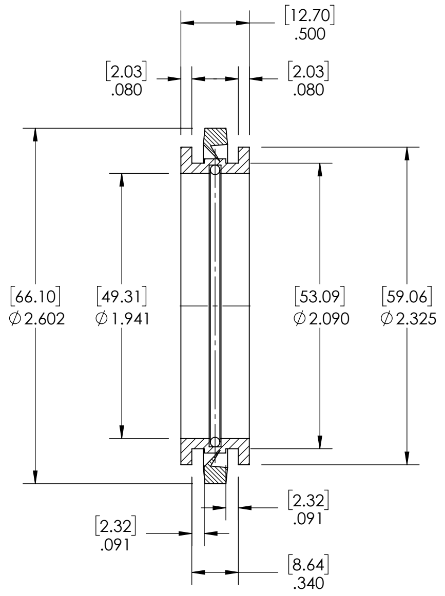
SECTION VIEW A-A
