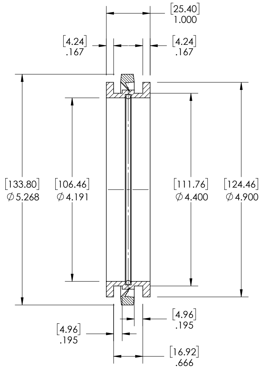
SECTION VIEW A-A
