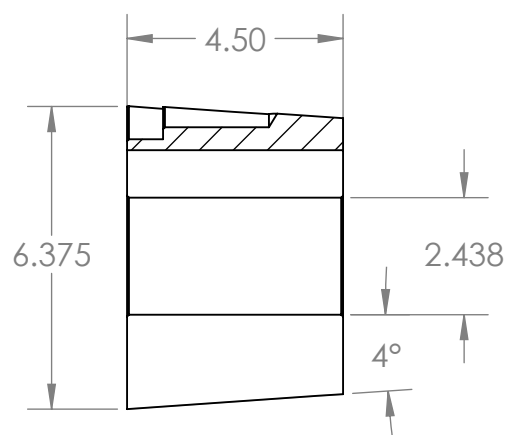
SECTION B-B
