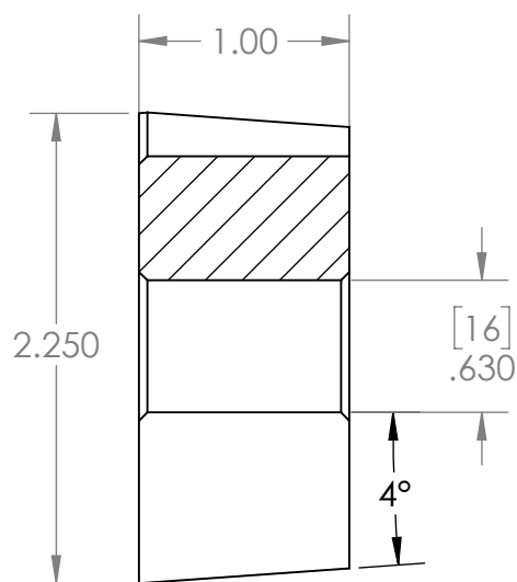
SECTION B-B
