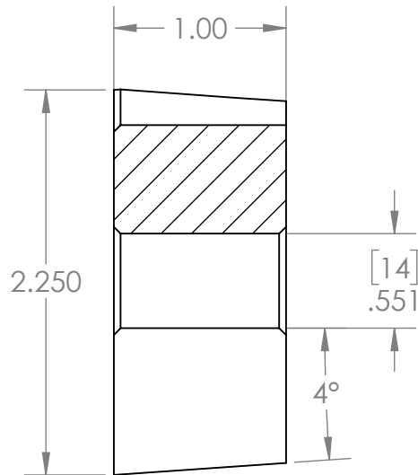
SECTION B-B
