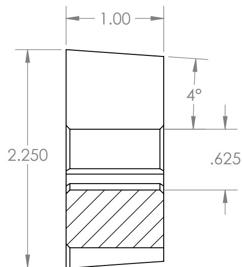
SECTION B-B
