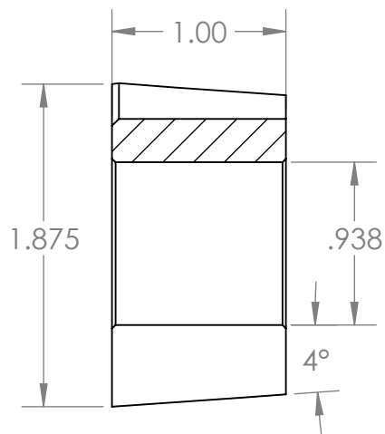
SECTION B-B
