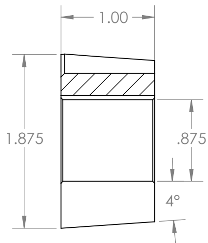
SECTION B-B
