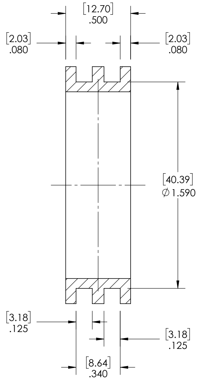
SECTION VIEW A-A
