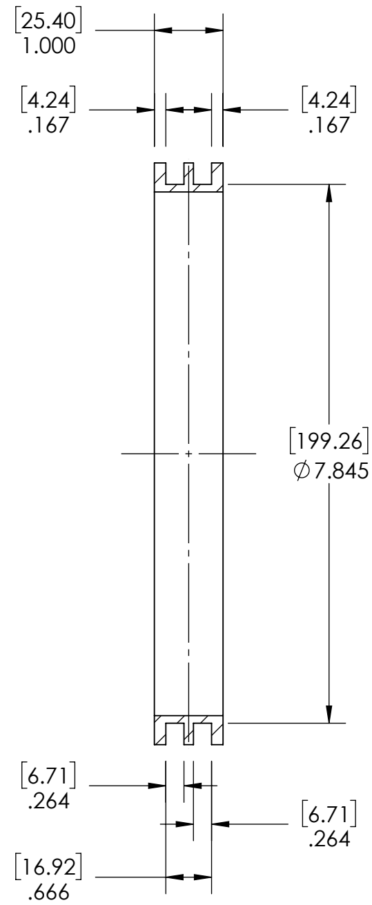
SECTION VIEW A-A
