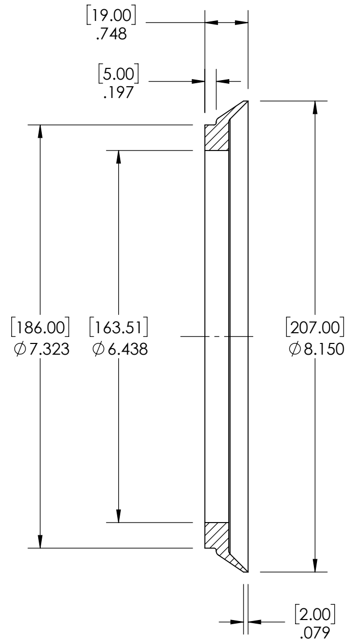
SECTION VIEW A-A
