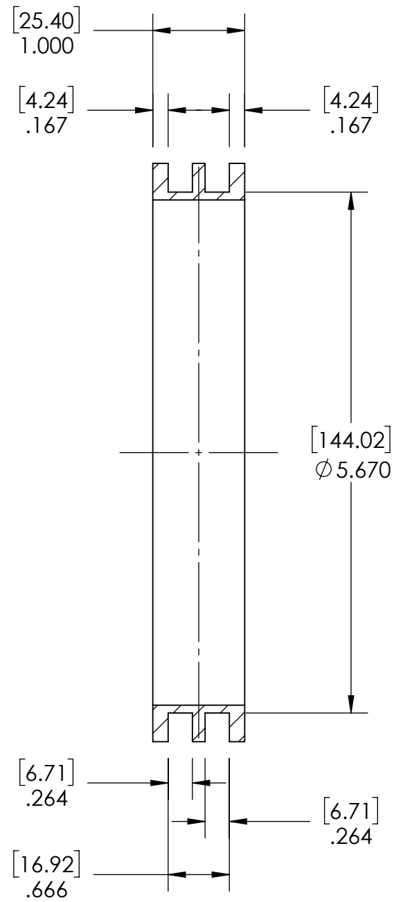
SECTION VIEW A-A
