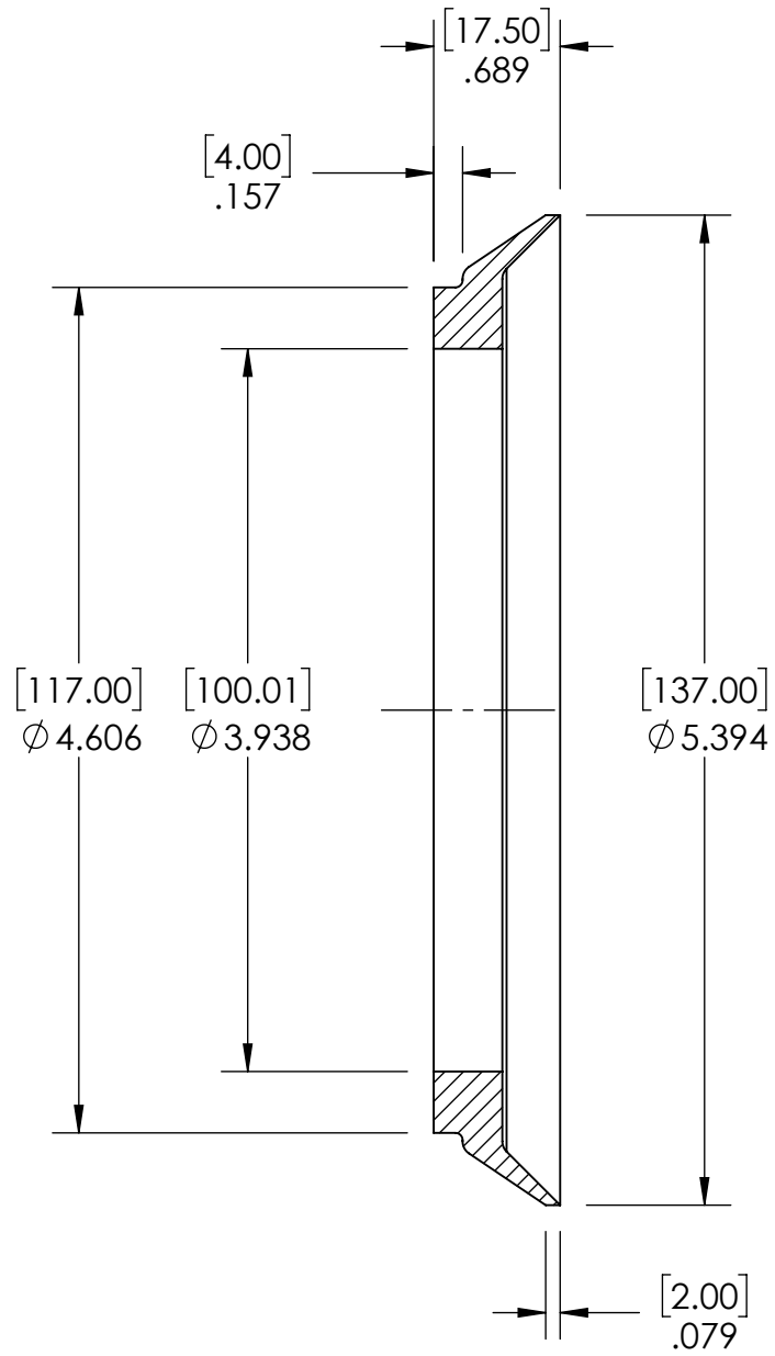
SECTION VIEW A-A
